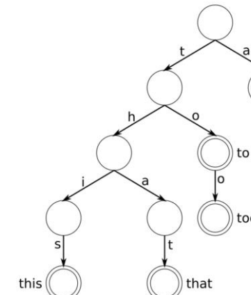
Fig. 4: Prefix tree containing words "to", "to", "to", "this" and "that".
