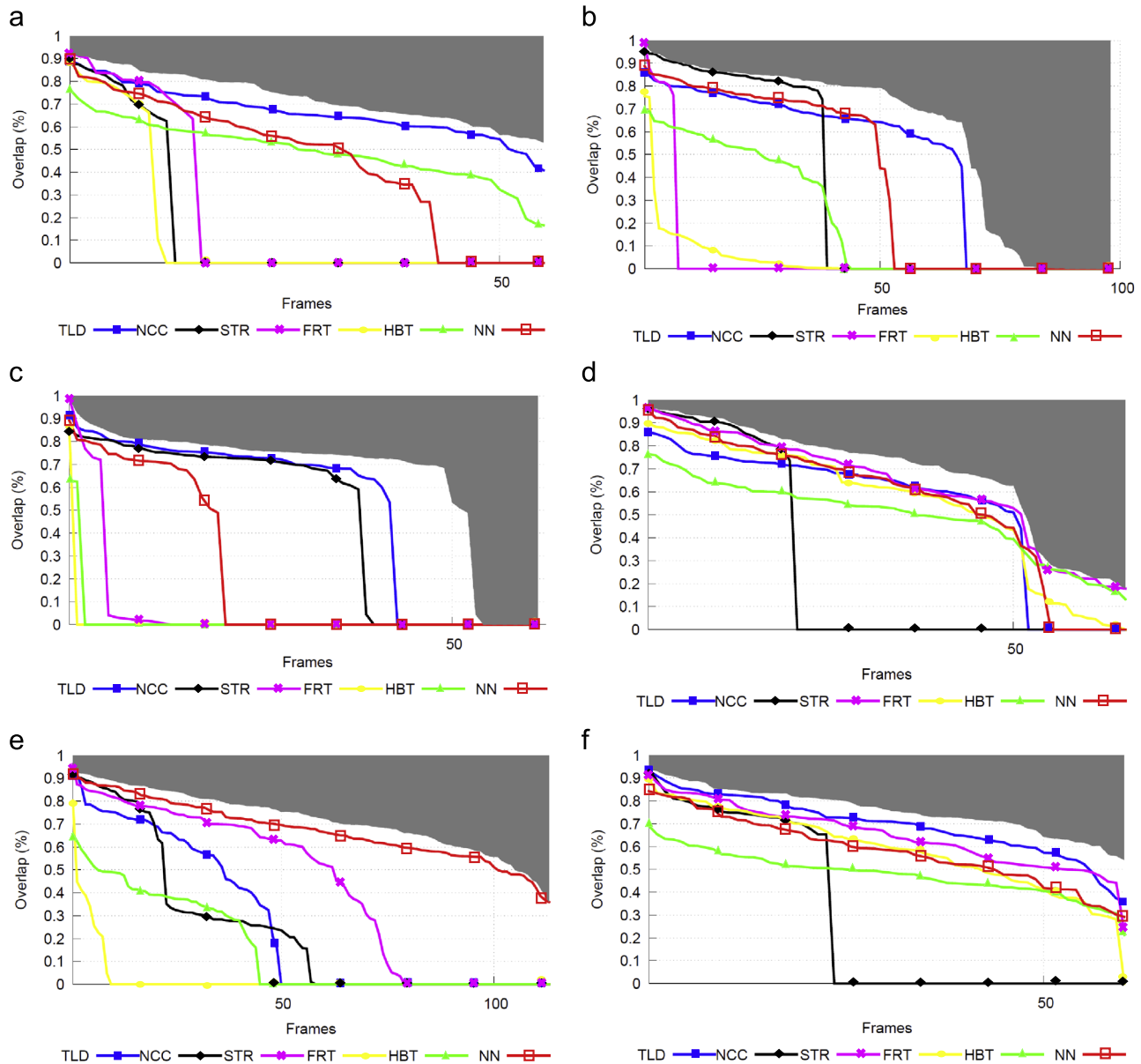
Fig. 6. Overlap percentage between predicted bounding box and ground truth in our tracking evaluation. The plots represent data in the form of a survival curve, meaning that if a tracker scores a 0.5 overlap at frame 50, its overlap is \geq 0.5 in at least 50 frames. The videos feature the following settings and main challenges: (a) indoor, crowded sequence; (b) outdoor, low camera motion; (c) indoor, high camera motion; (d) indoor, controlled environment; (e) indoor, first person motion; (f) indoor, poor lighting. The frame number refers to the frame which had its ground truth for the subject's bounding box annotated, which is a frame out of 5. Best viewed in colors. (For interpretation of the references to color in this figure caption, the reader is referred to the web version of this paper.)
